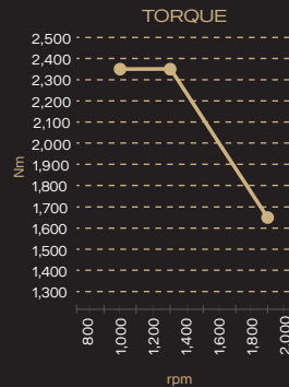
DC13 146 500 Euro 5
